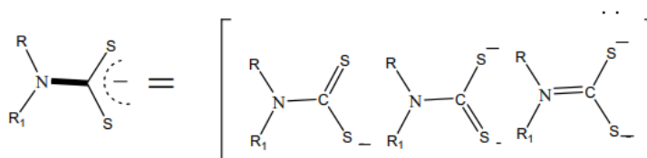
Fig-Resonance form of dithiocarbamate metal complexes
